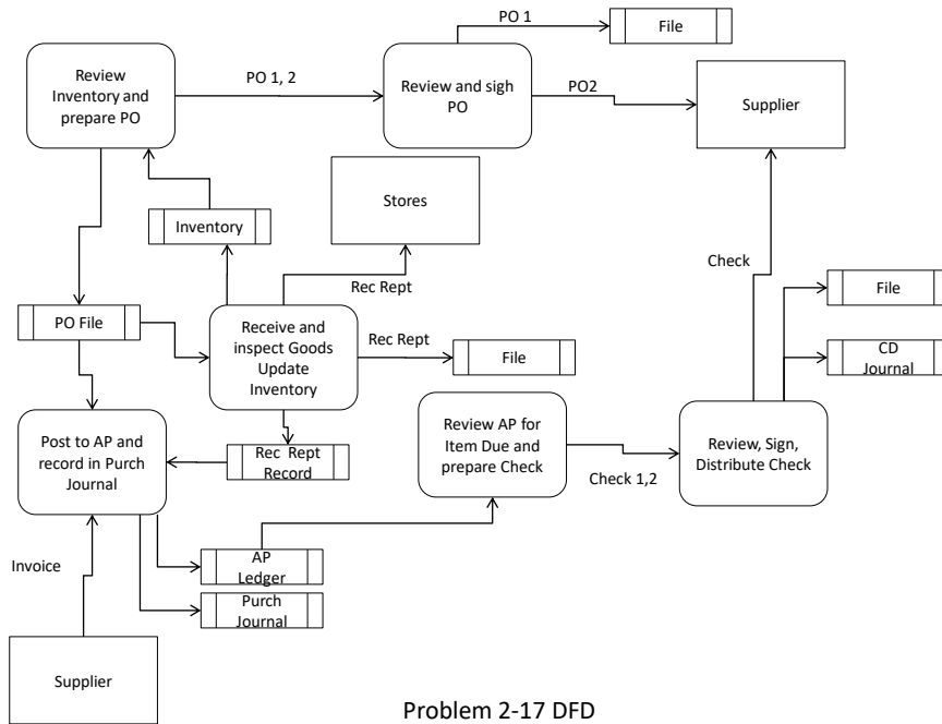
Problem 2-17 DFD
