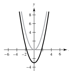
Vertical shift three units downward
